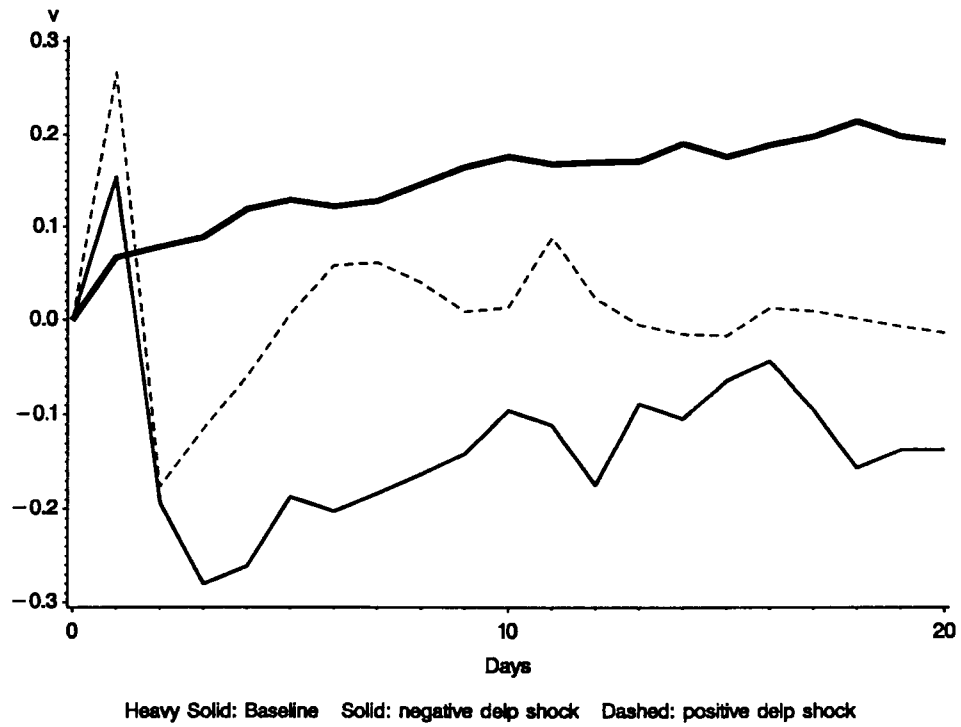
Figure 6: Impulse Responses of Volatility and Volume to Pure \Delta p Shock (Type B)
