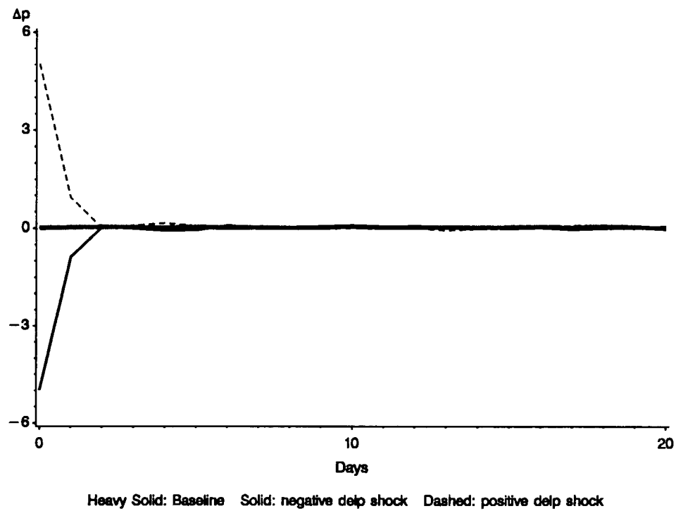
Figure 1: Impulse Response of \Delta p to \Delta p Shock in Univariate Fit
