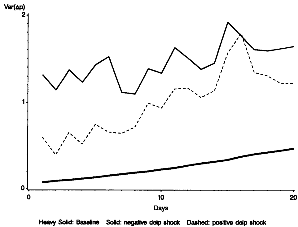
Figure 2: Impulse Response of Volatility to \Delta p Shock in Univariate Fit
