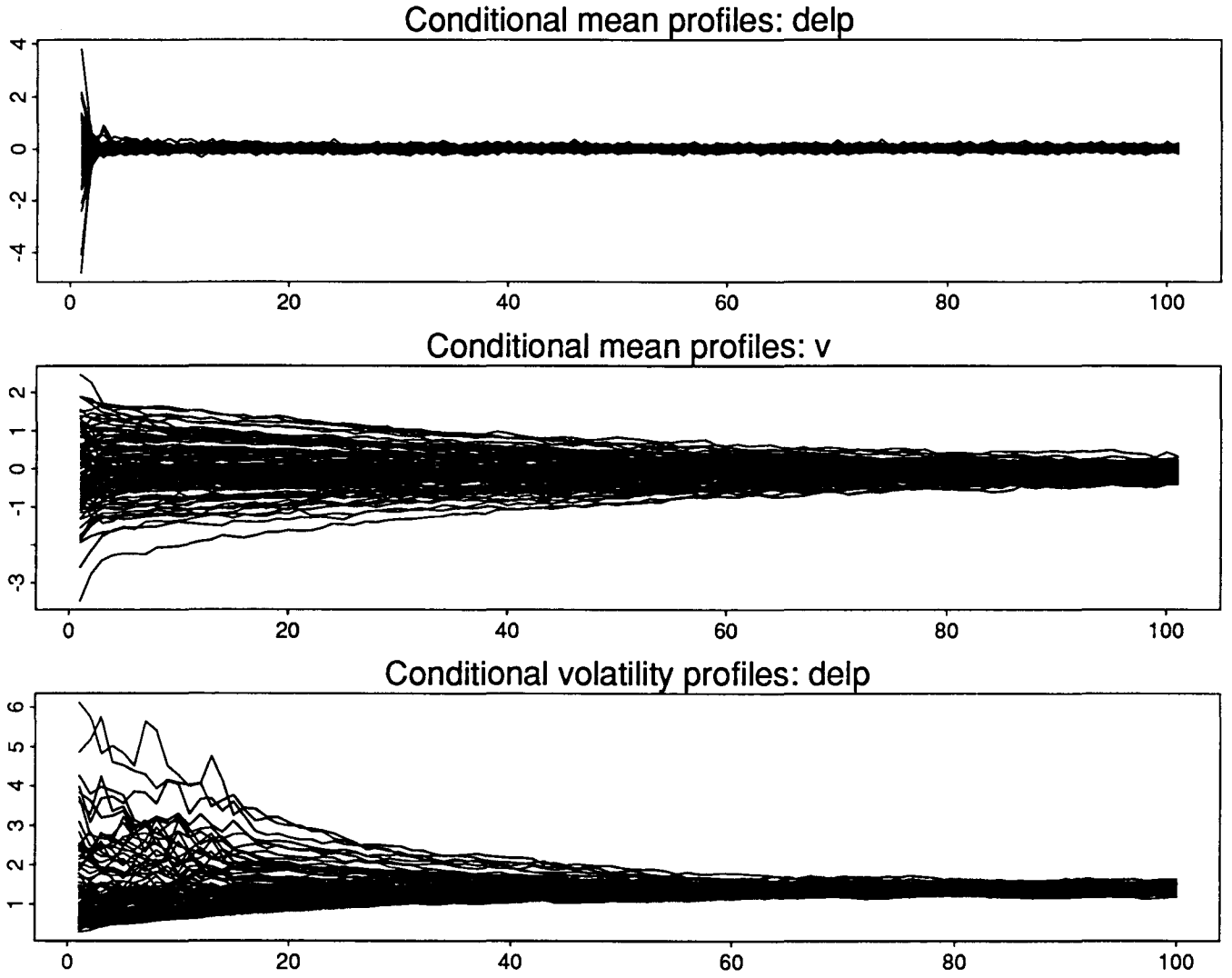
Figure 10: Profiles: \{\Delta \hat{p}_j(x_t)\}_{j=1}^{100} , \{\hat{v}_j(x_t)\}_{j=1}^{100} , \{\hat{\mathcal{V}}_{\Delta p, j}(x_t)\}_{j=1}^{100} , t = 28, 156, \dots, 16028
