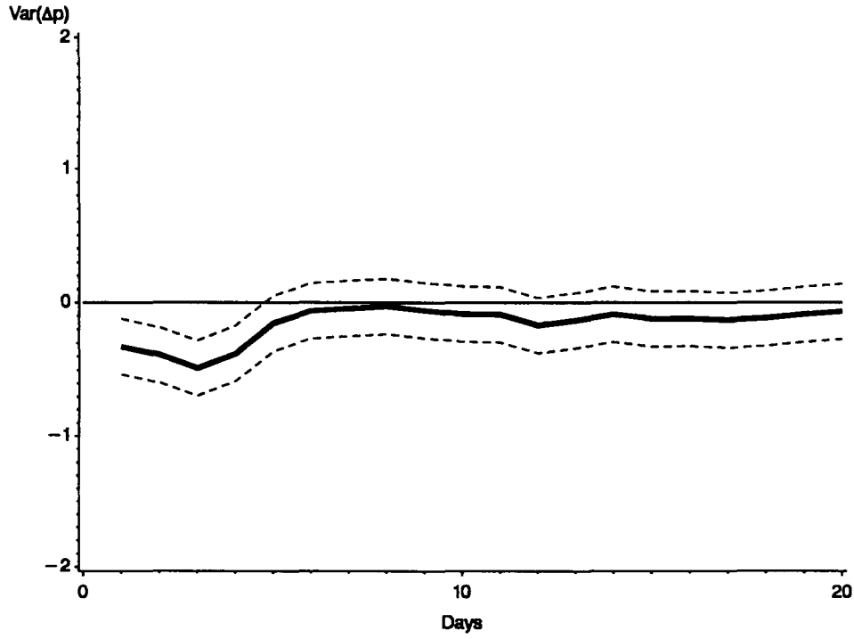
Figure 8: 95% Band for Differential Response of Volatility to \Delta p and v Shock (Type A)
