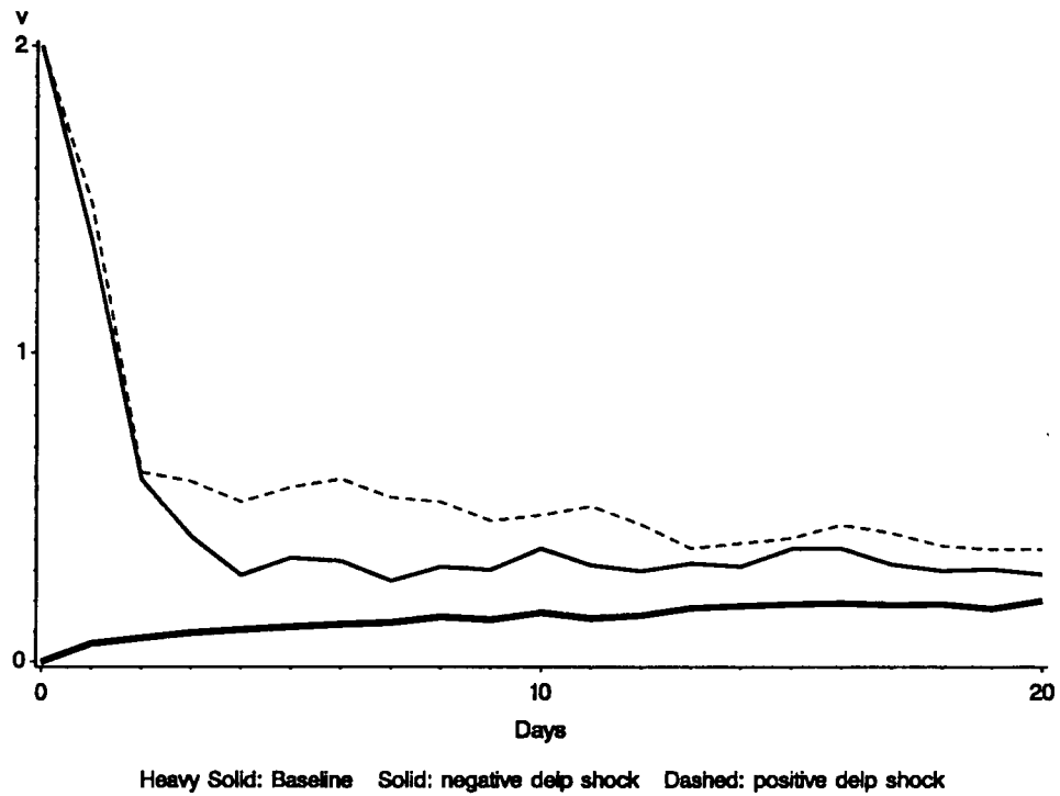
Figure 5: Impulse Responses of Volatility and Volume to \Delta p and v Shock (Type A)
