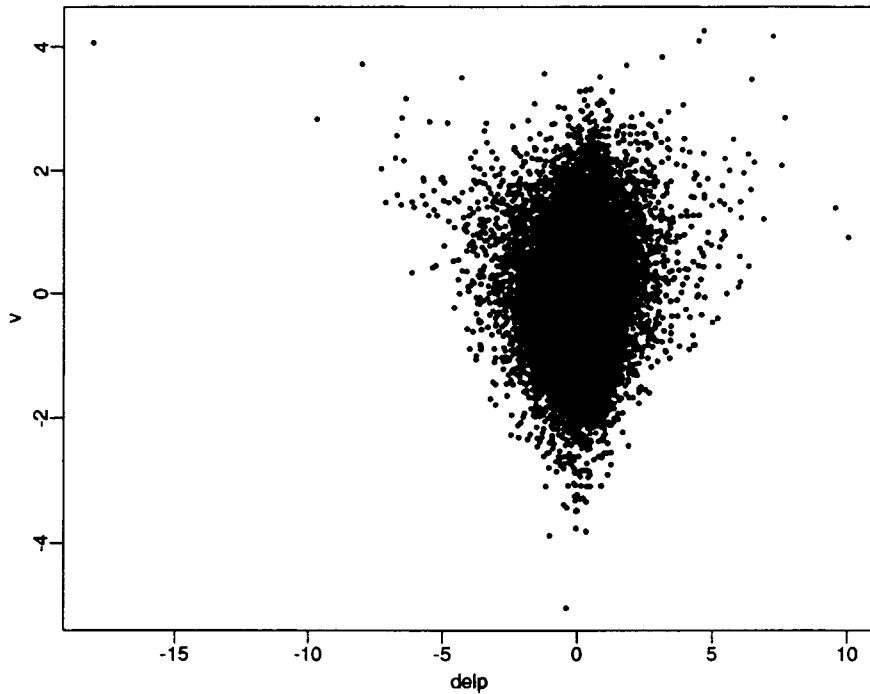
Figure 3: Scatter Plot of Adjusted (\Delta p, v) Data
