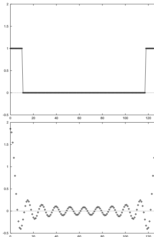
A pulse and its discrete fourier transform, output from the example program.
